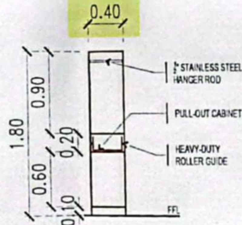
SECTION - (A)
