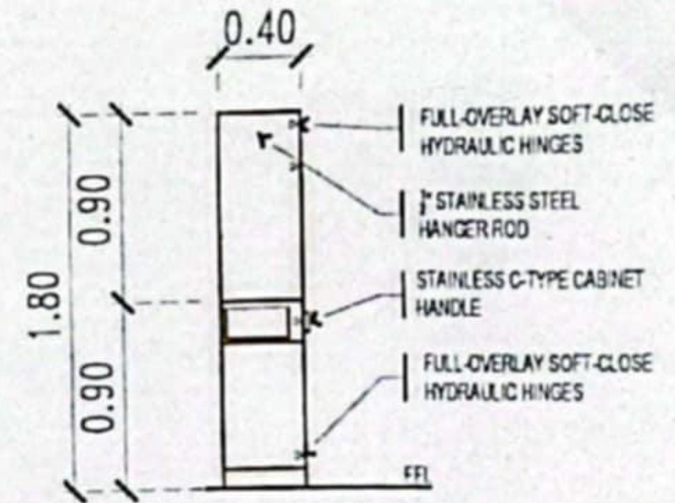
SECTION - (B)
