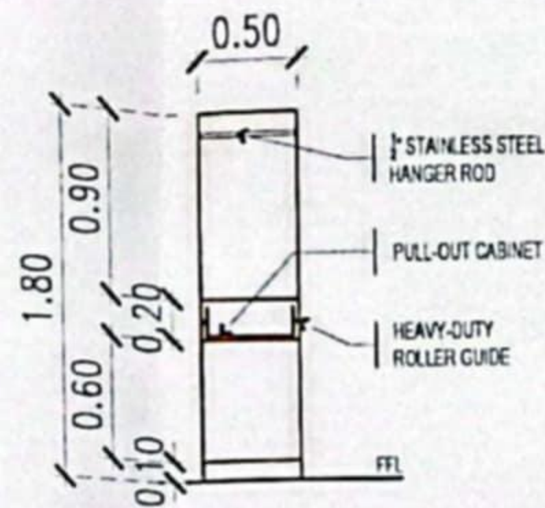
SECTION - (A)
